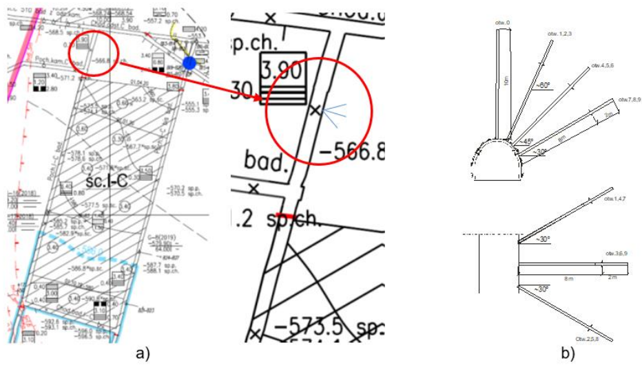
Site of the stress measurements (a) and boreholes to measure characteristic hydrofracturing pressures (b).
