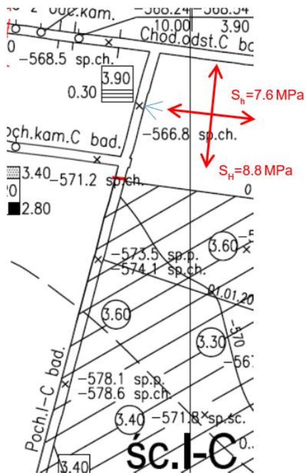
Directions and values of horizontal stresses obtained from measurements in gate 1-C in seam 501.
